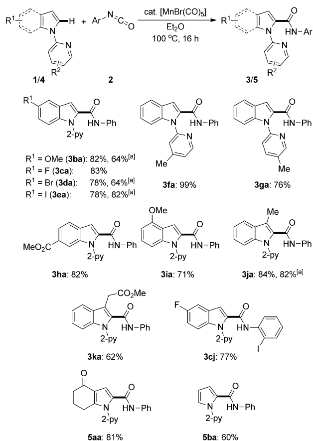
Scheme 2. Manganese-catalyzed C–H activation with indoles 1 and pyrroles 4 . [a] n\text{Bu}_2\text{O} used as solvent.
