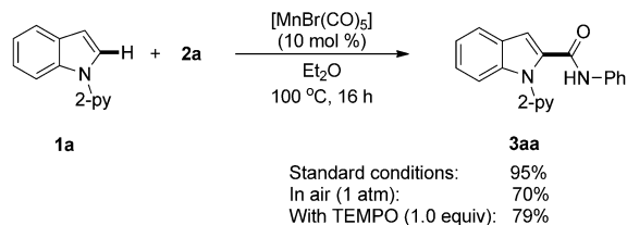
Scheme 5. Evidence supporting an organometallic activation mode for the C–H functionalization process.
