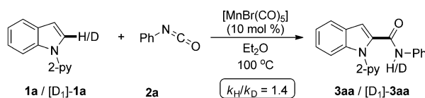
Scheme 3. Studies with isotopically labeled compounds.
