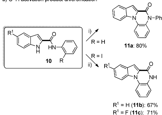
Scheme 7. Diversification of C–H activation products. Reagents and conditions: i) 1-Fluoro-2-nitrobenzene, CS_2CO_3 , CH_3CN , 90^\circ C , 12 h. ii) CuI (cat.), L -proline (cat.), NaH, DMF, 150^\circ C , \mu w , 5 min.
