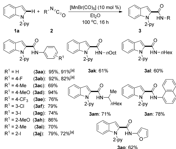
Scheme 1. Manganese-catalyzed C–H aminocarbonylation with isocyanates 2 . [a] n\text{Bu}_2\text{O} used as solvent.
