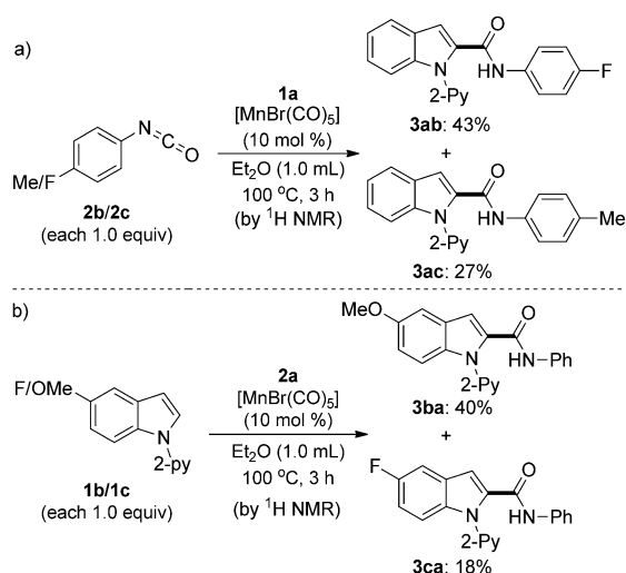
Scheme 4. Intermolecular competition experiments.
